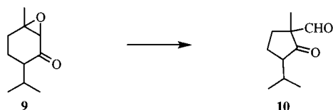
Scheme 7. Rearrangement of piperitone oxide ( 9 ) to 3-isopropyl-1-methyl-2-oxocyclopentane-1-carbaldehyde ( 10 )
